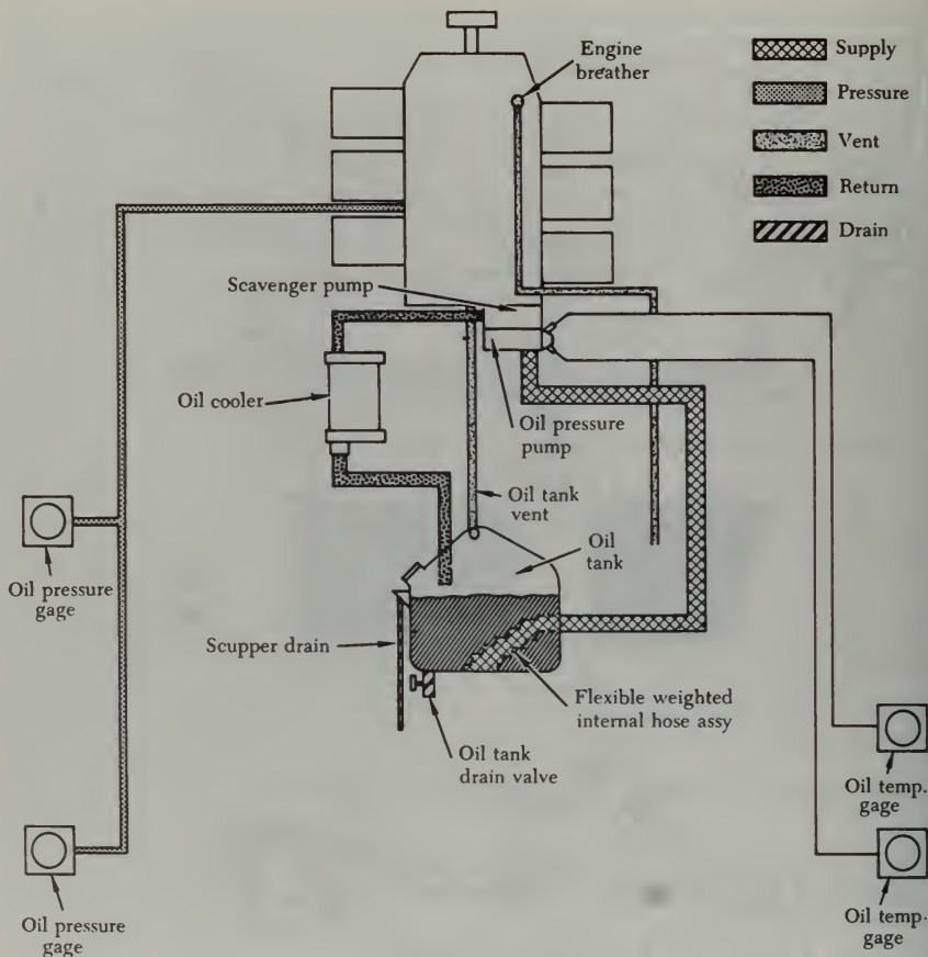
FIGURE 6-11. Oil system schematic.
